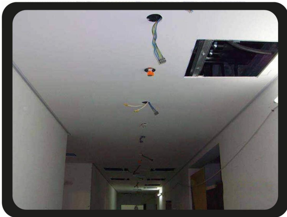
Installation of recessed Sprinkler
