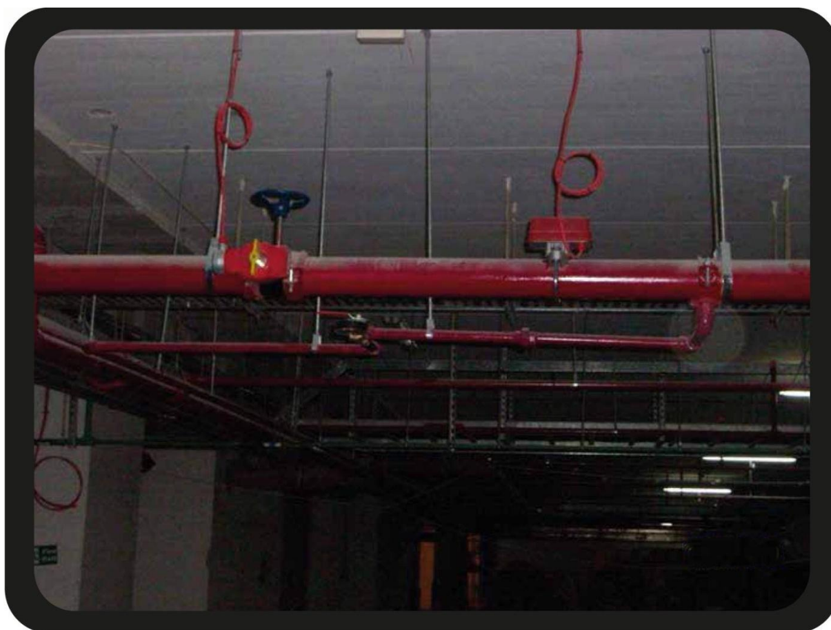
Header Pipes with Zone Control Valve
