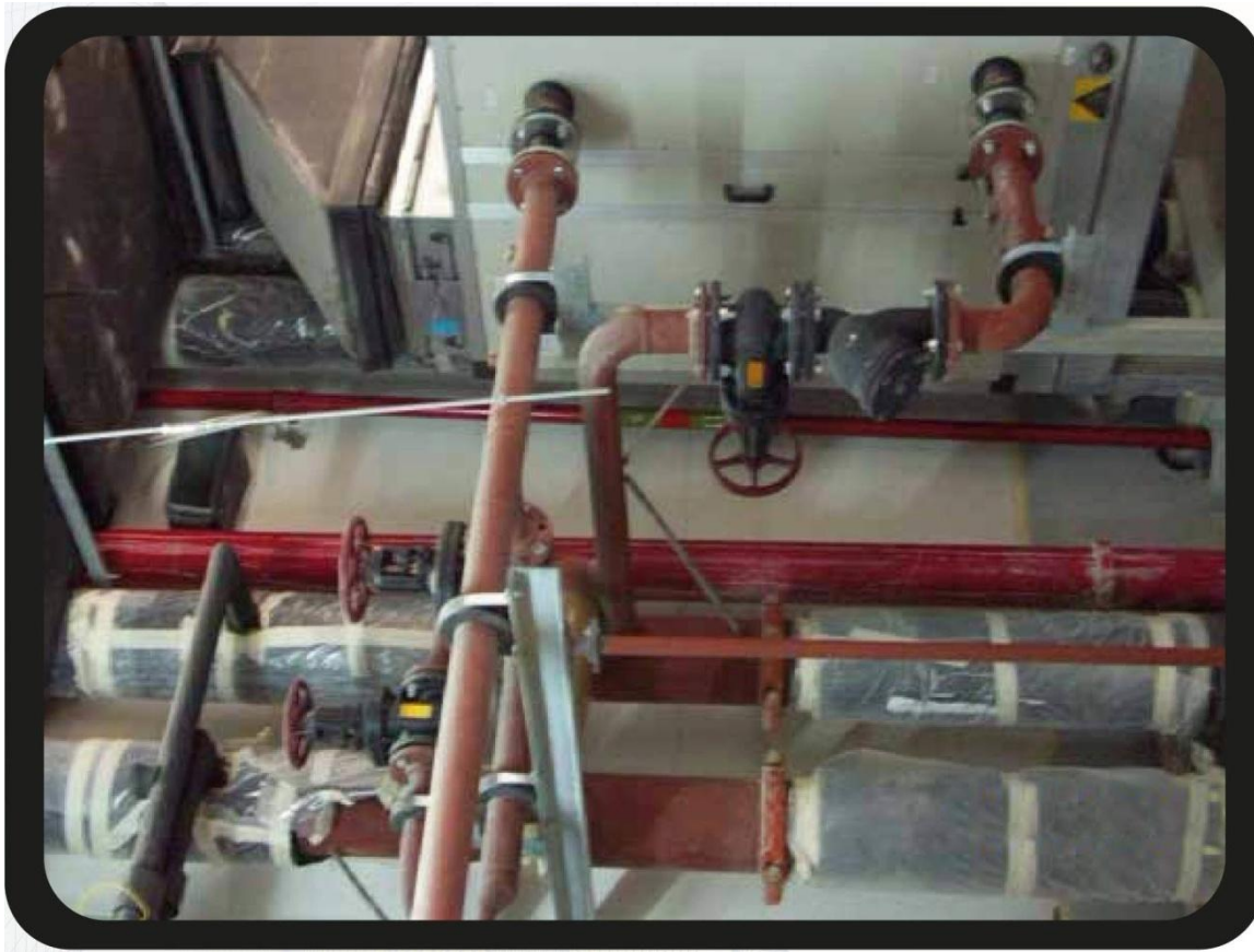
Wet Riser with drain line
